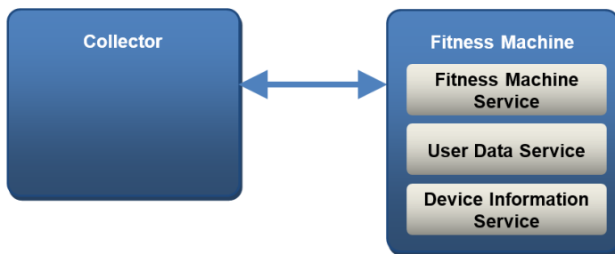
Figure 2.1: Relationships between services and profile roles for the Fitness Machine profile
